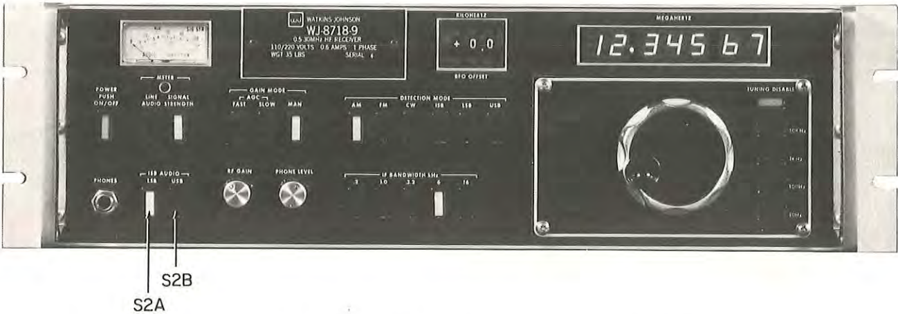
Figure 7-2. WJ-8718-9 HF Receiver Front View, Location of Components
