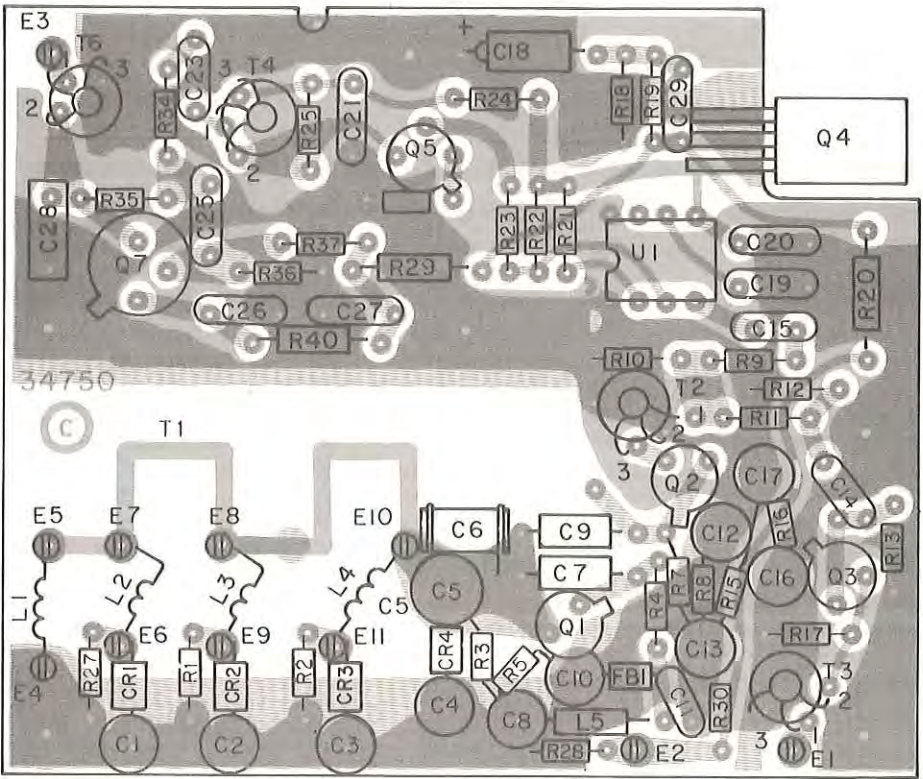
Figure 5-25. Part 34750 1st LO Voltage Controlled Oscillator (A5A1A1A1)
