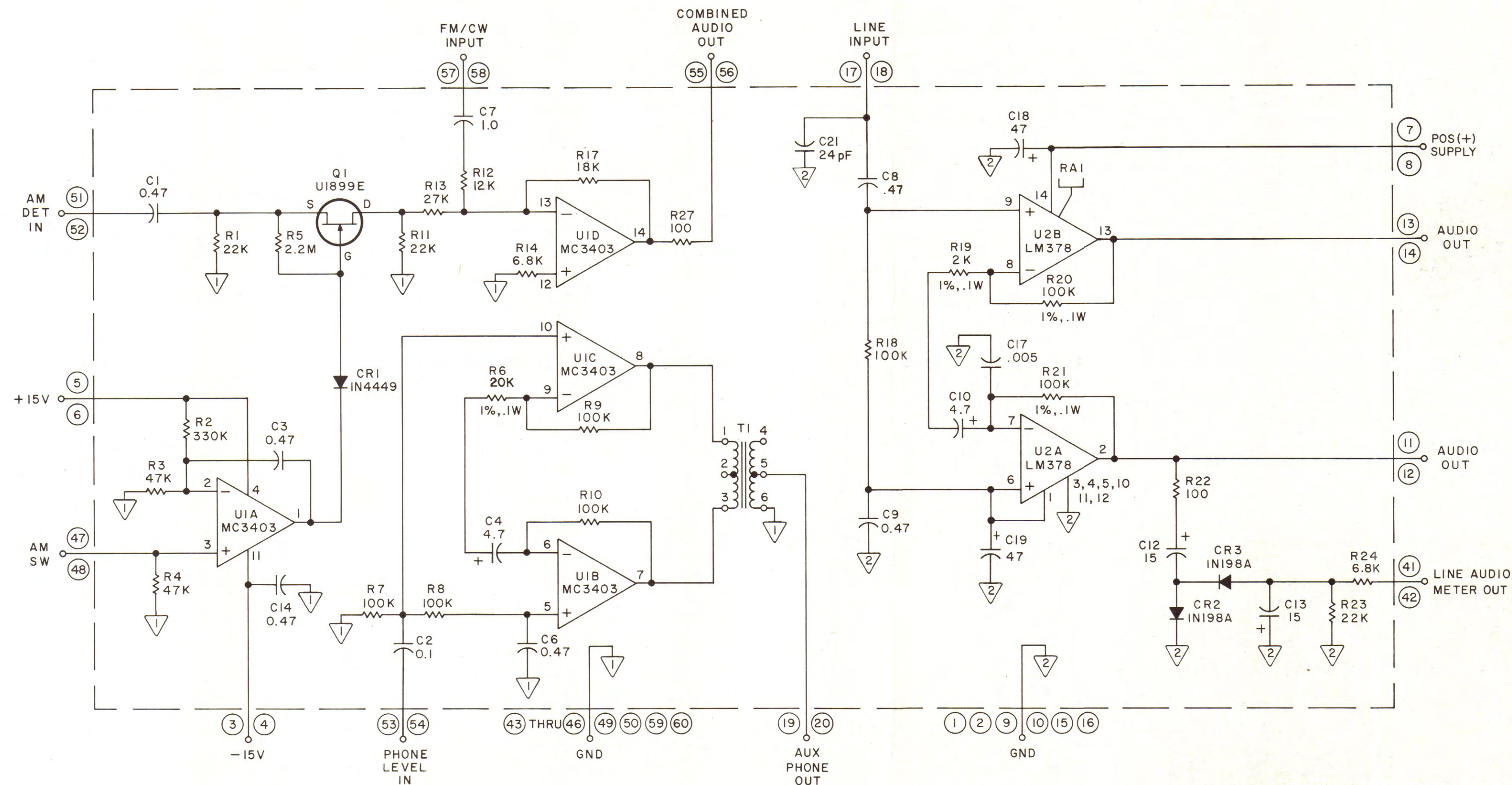
Figure 7-7. Type 746001 Audio Amplifier (A4A10), Schematic Diagram 480089
