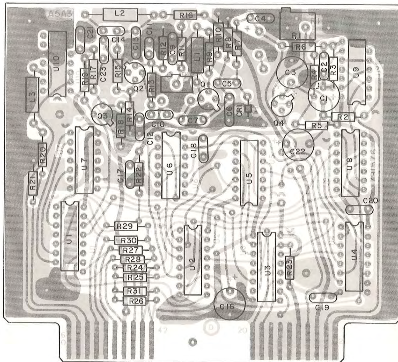
Figure 5-28. Type 791576 BFO Synthesizer (A5A3), Location of Components
