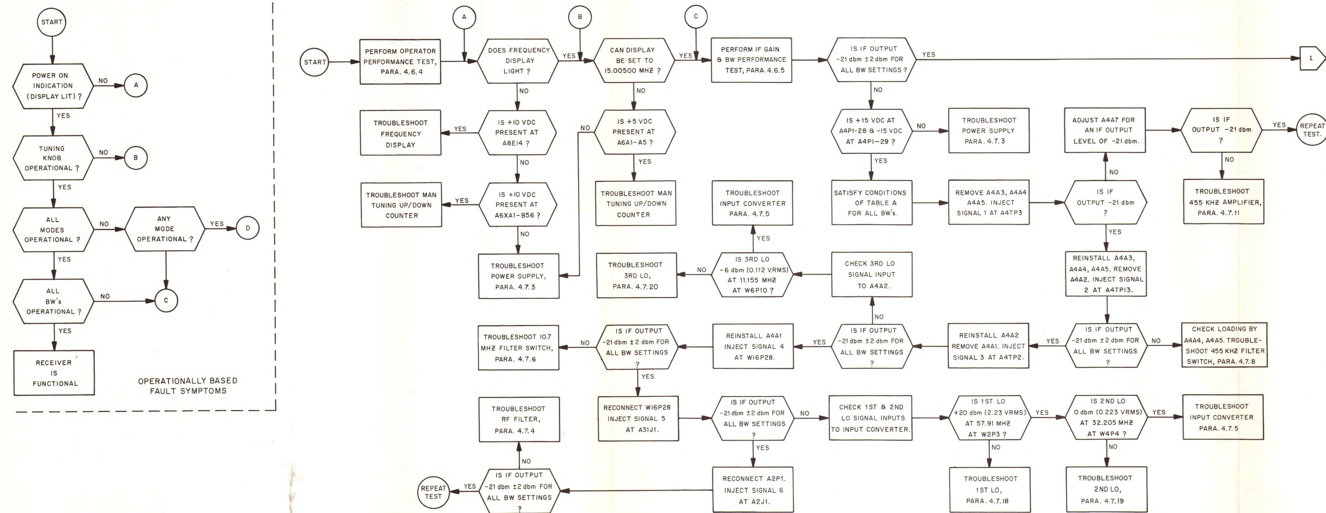
Figure 4-1a. Corrective Maintenance Flowchart
