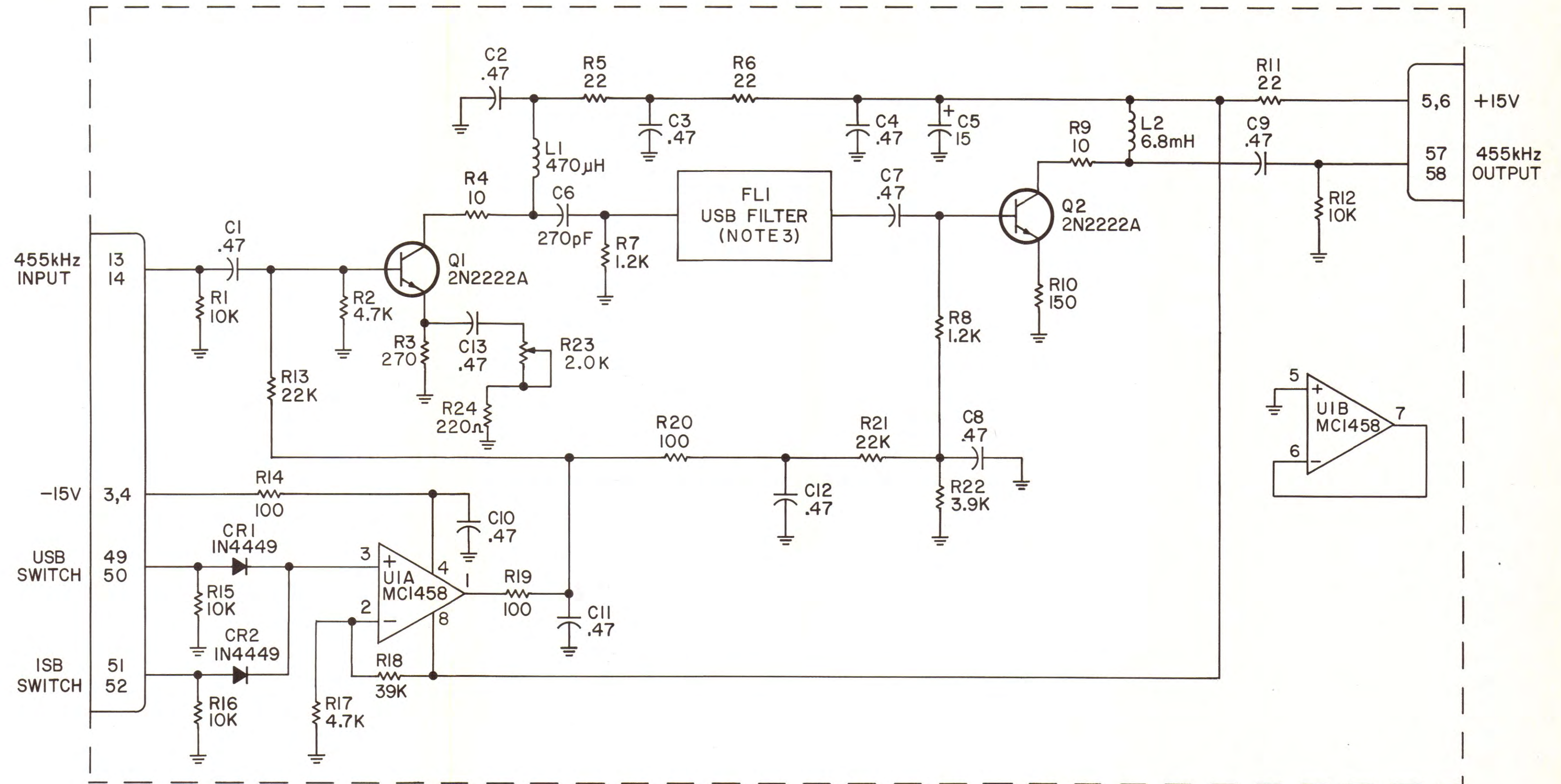
Figure 6-6a. Type 791596 USB Filter Switch Option (A4A4) Schematic Diagram 480102 (Product Improvement)
