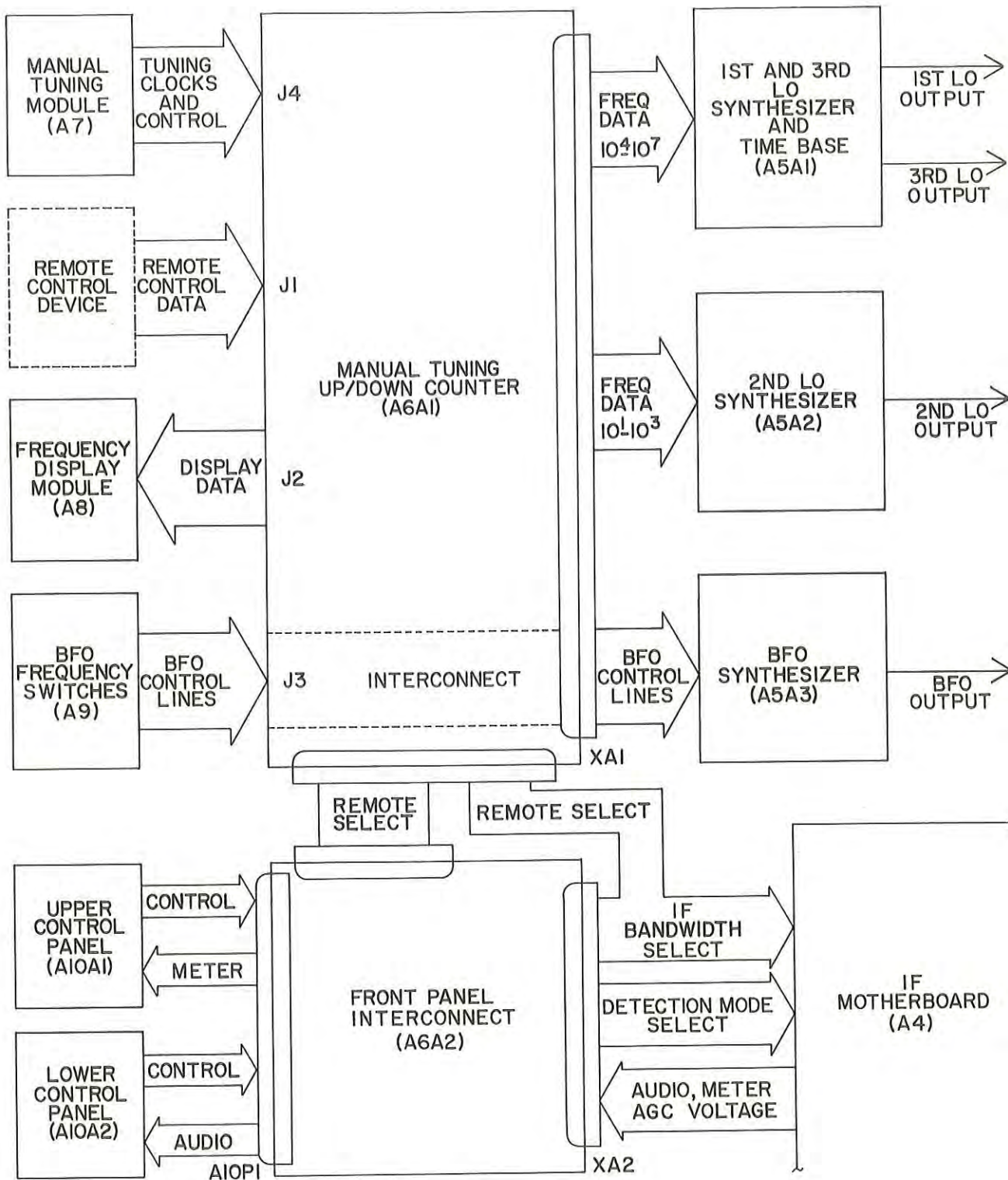
Figure 3-21. Digital Section Functional Block Diagram
