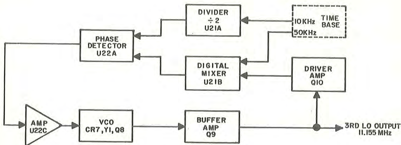
Figure 3-12. 3rd LO Functional Block Diagram
