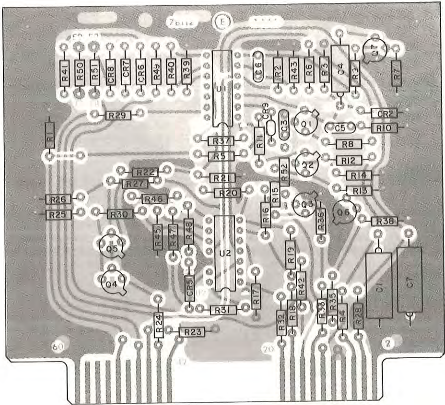
Figure 5-17. Type 78112 AGC Amplifier (A4A6), Location of Components
