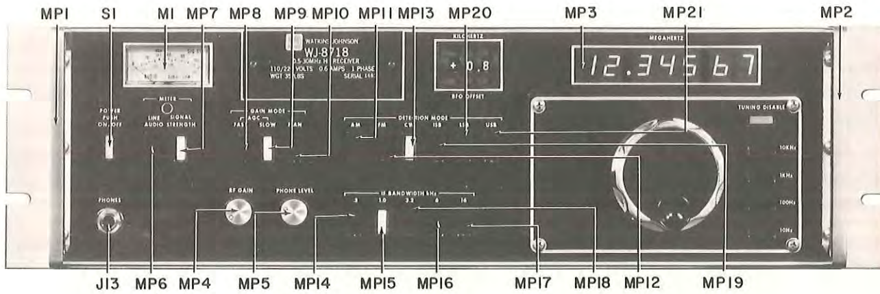
Figure 2-2. WJ-8718 HF Receiver, Front Panel View
