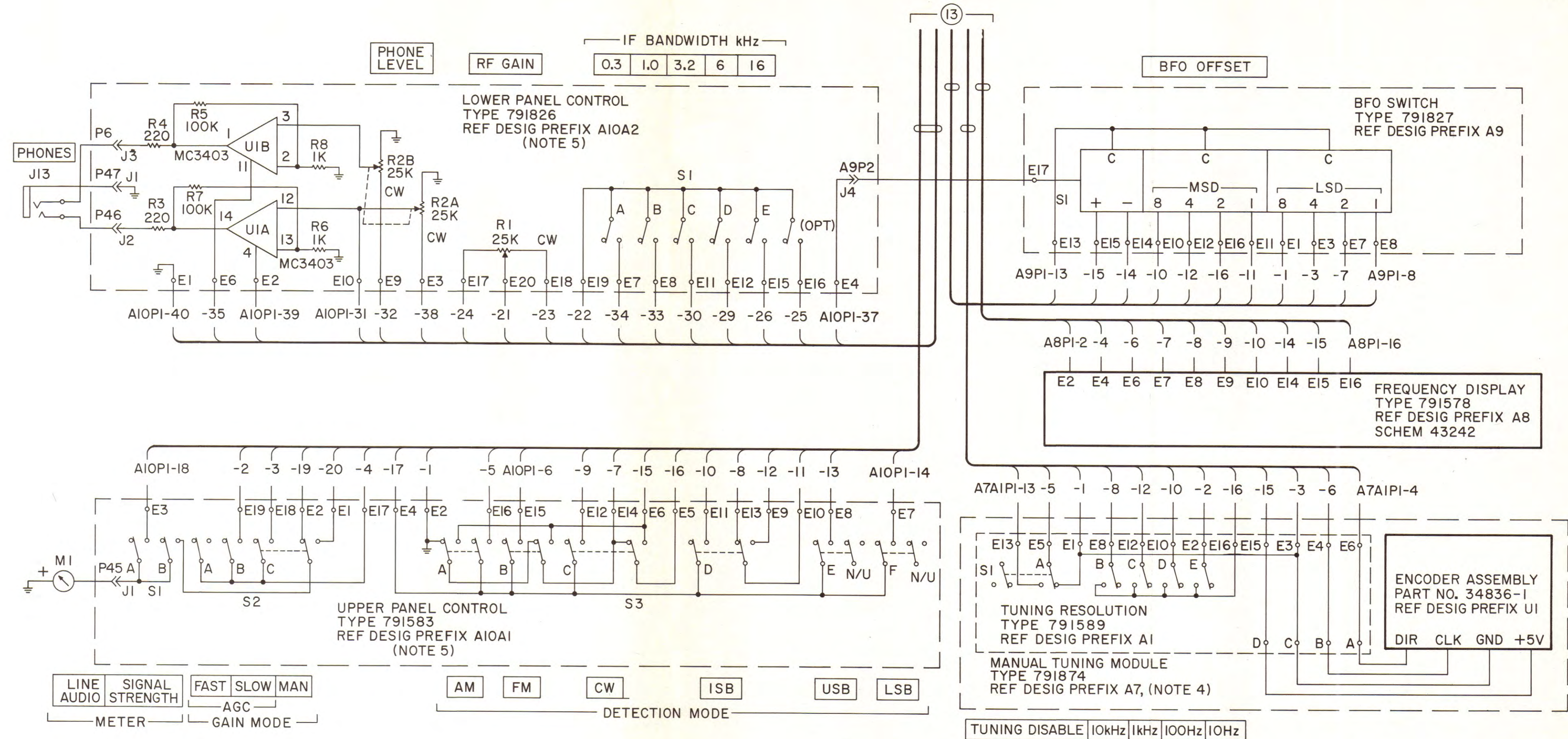
Figure 6-21. Type WJ-8718 HF Receiver Main Chassis, Schematic Diagram 580032 (Sheet 1 of 6 and Sheet 5 of 6) 6-41
