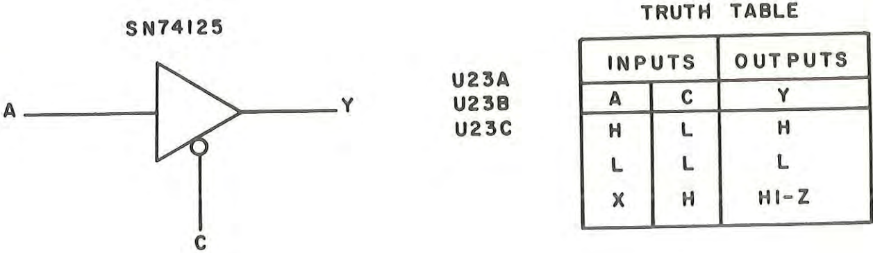
Figure 3-11. Tri-State Buffers
