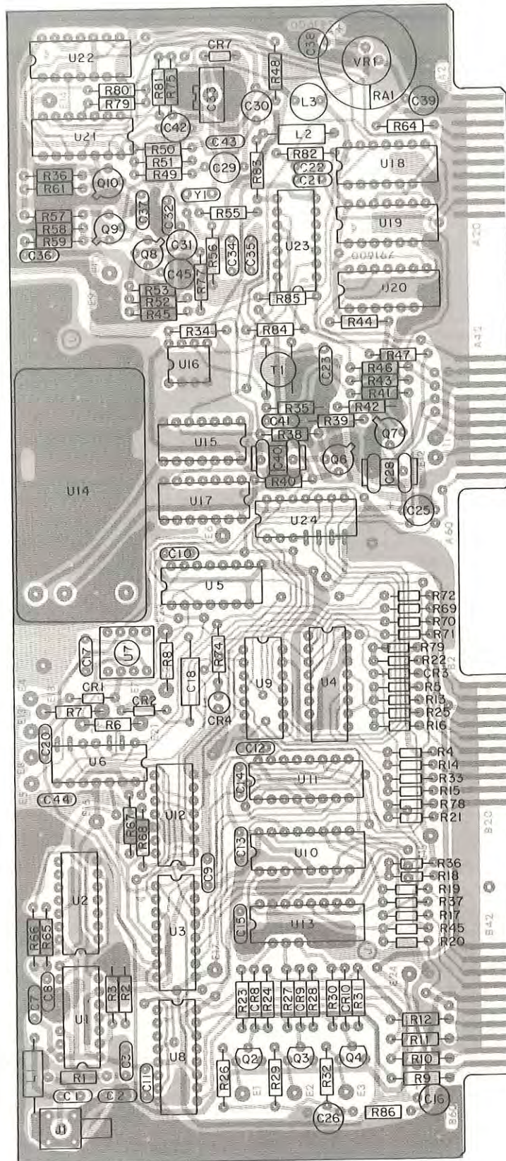
Figure 5-26. Type 791600 1st and 3rd LO Synthesizer (A5A1A2), Location of Components
