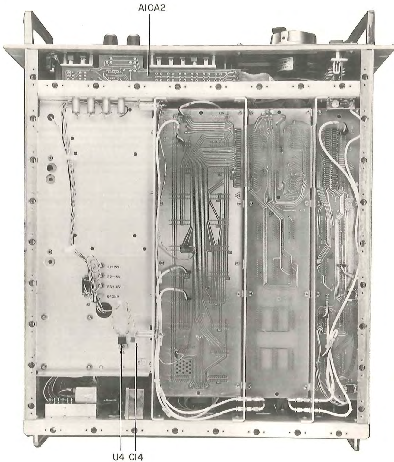
Figure 7-4. WJ-8718-9 HF Receiver Bottom View, Location of Components
