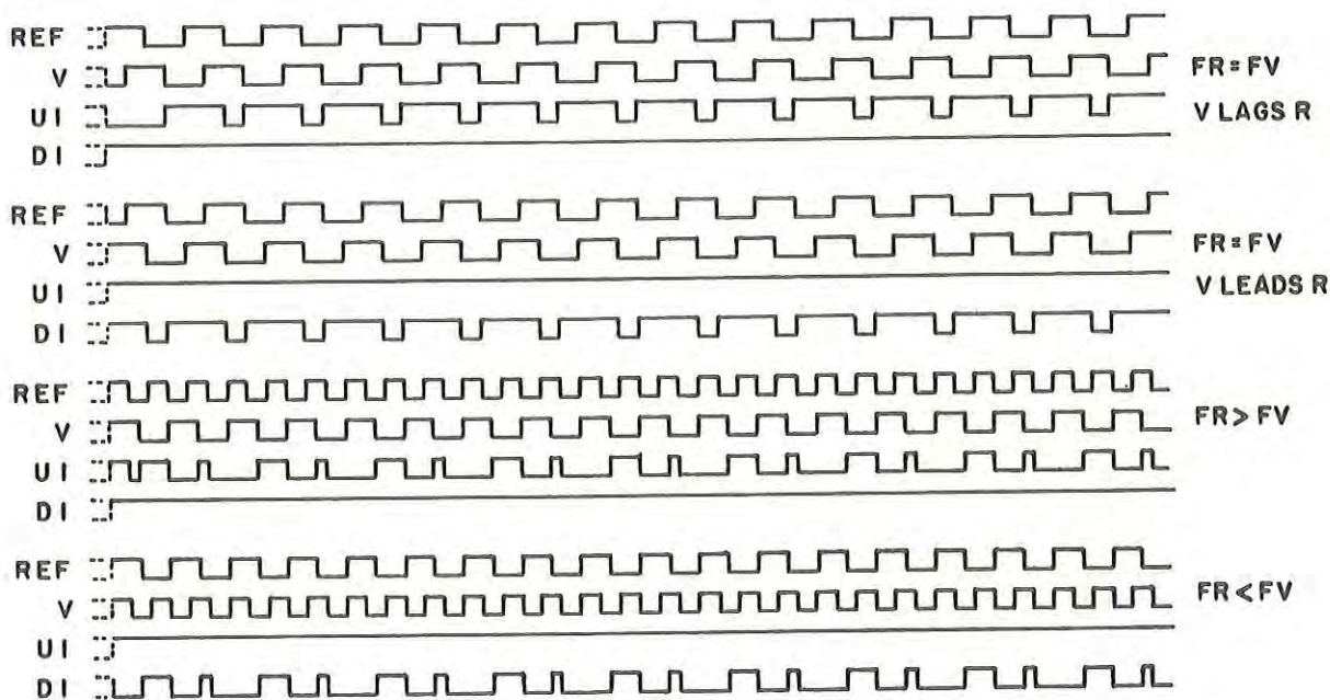
Figure 3-9. Phase Detector Timing Diagram
