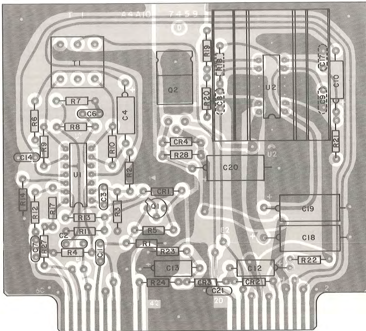
Figure 5-21. Type 7459 Audio Amplifier (A4A10), Location of Components
