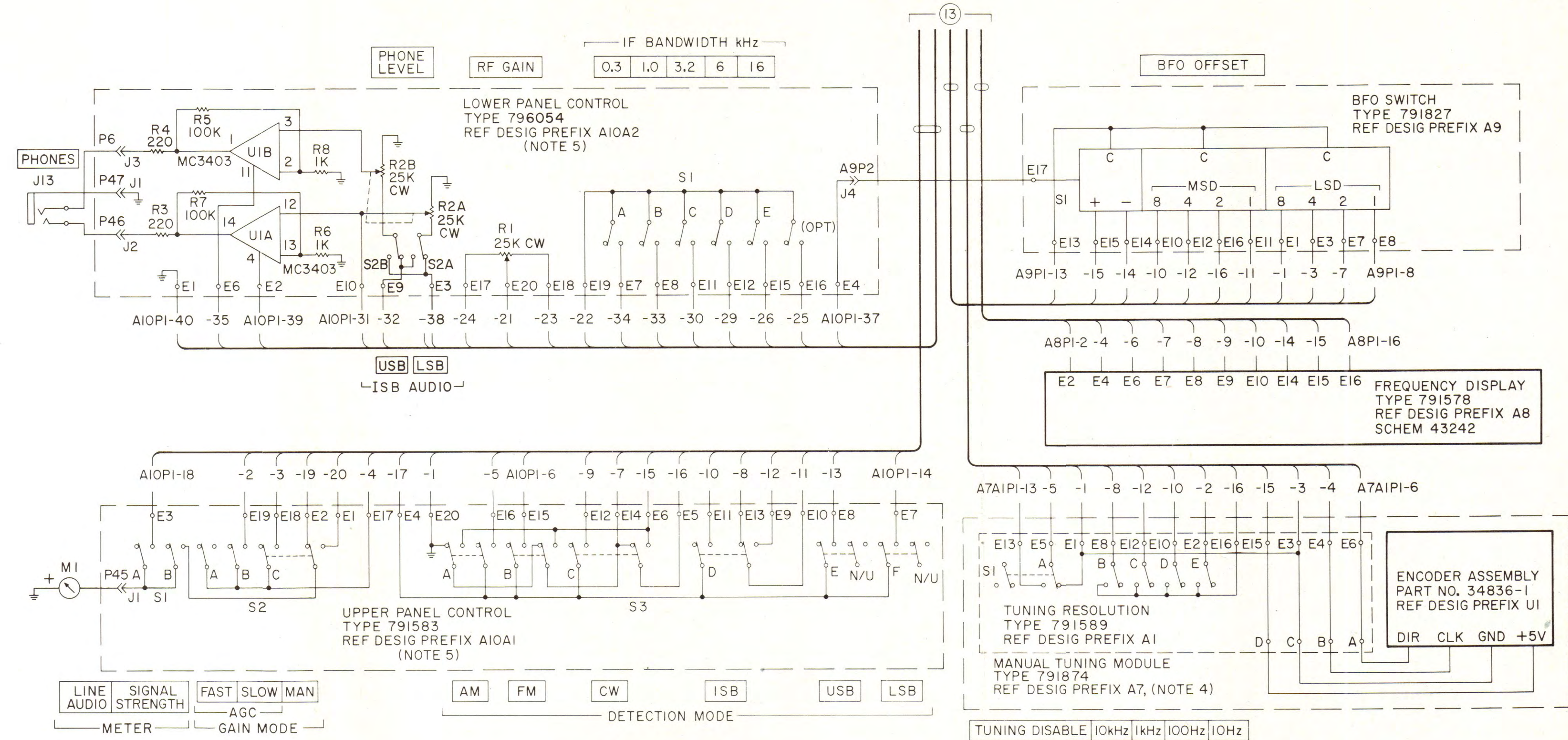
Figure 7-8. Type WJ-8718-9 HF Receiver Main Chassis Schematic Diagram 580032 (Sheet 1 of 6 and 5 of 6)
