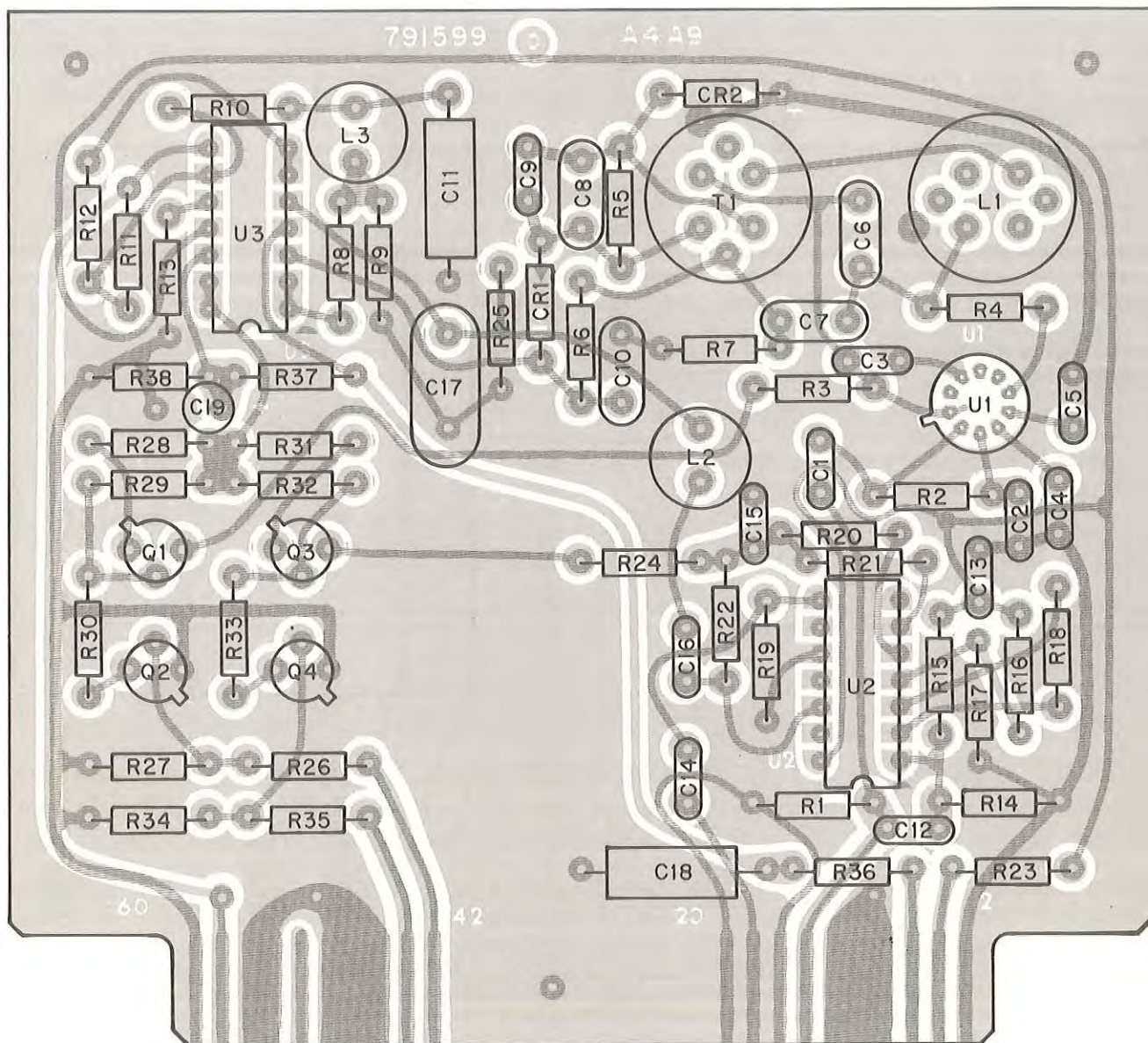
Figure 5-20. Type 791599 FM, CW, and SSB Detector (A4A9), Location of Components
