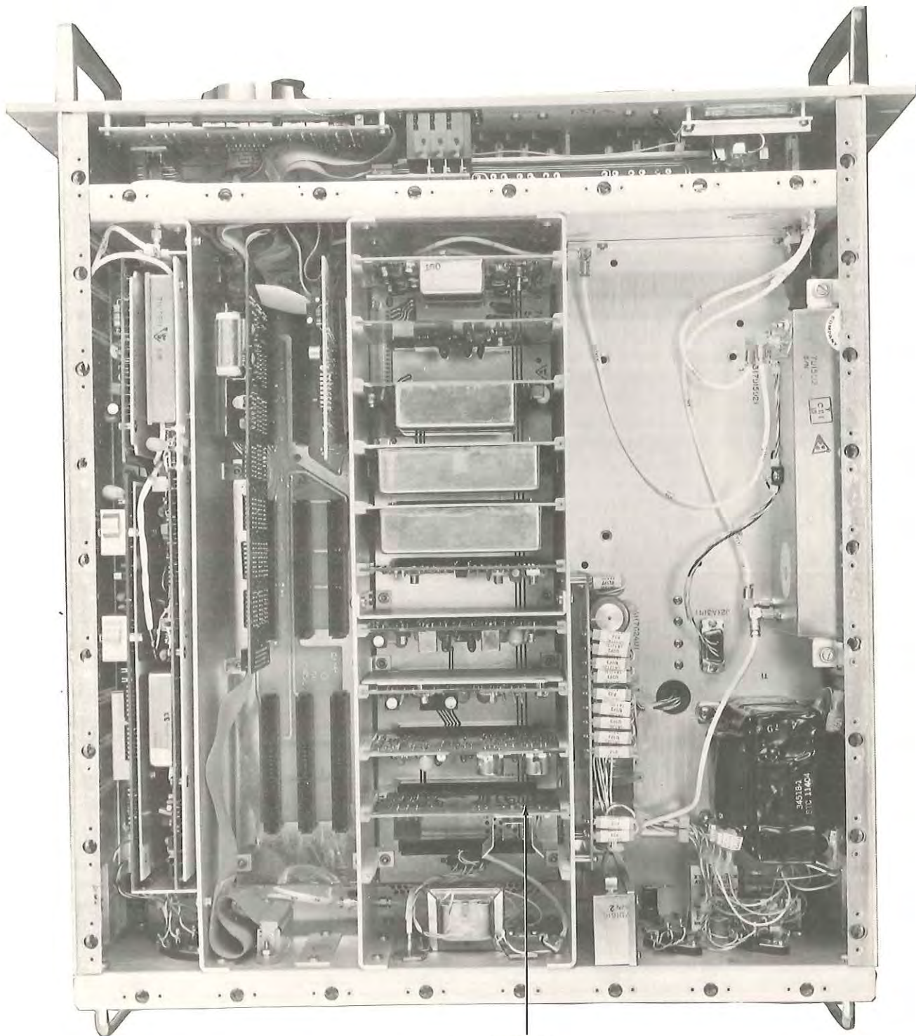
Figure 7-3. WJ-8718-9 HF Receiver Top View, Location of Components
