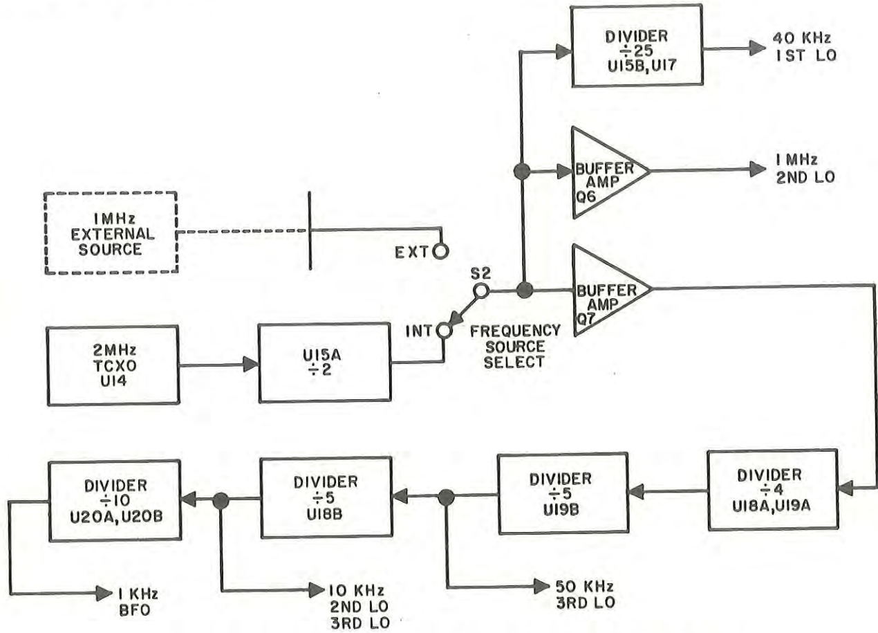
Figure 3-10. Time Base Circuits Functional Block Diagram
