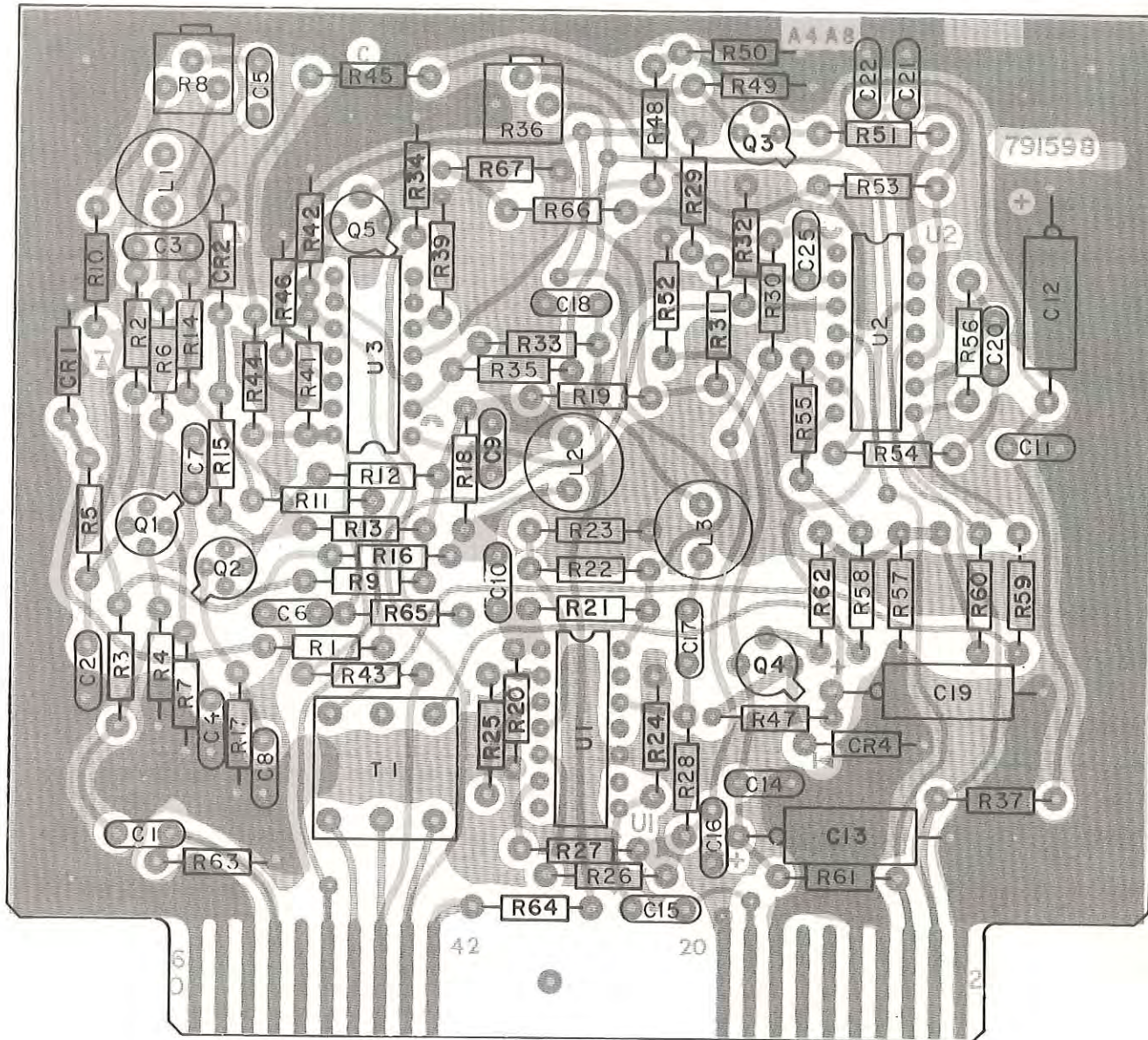
Figure 5-19. Type 791598 ISB Detector/Audio (A4A8), Location of Components
