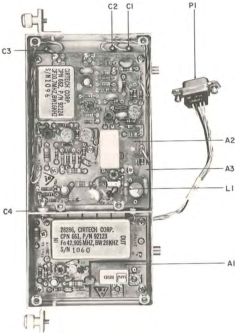
Figure 5-7. Type 791592-1 Input Converter (A3), Location of Components
