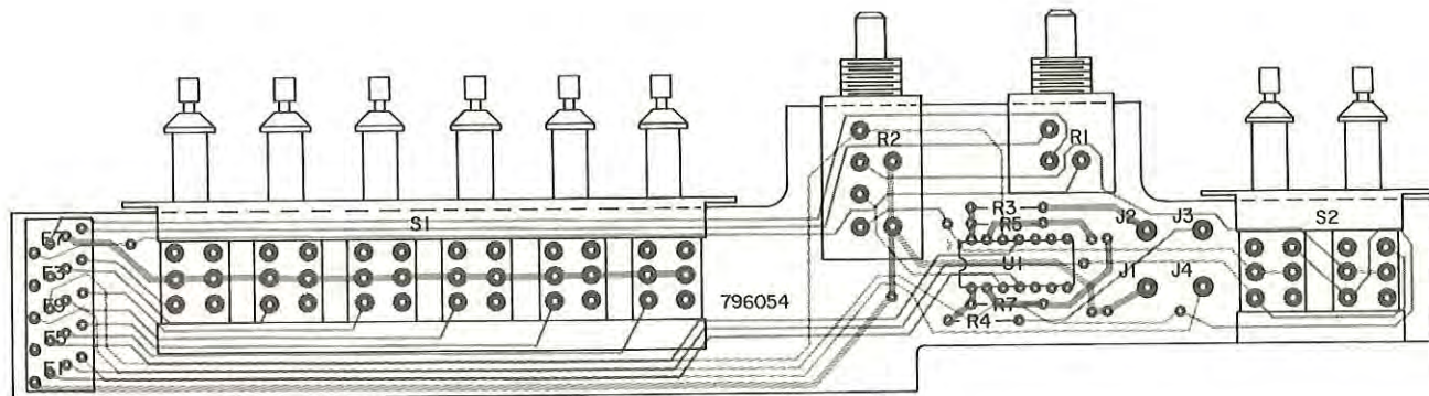
Figure 7-6. Type 796054 Lower Panel Control, Location of Components
