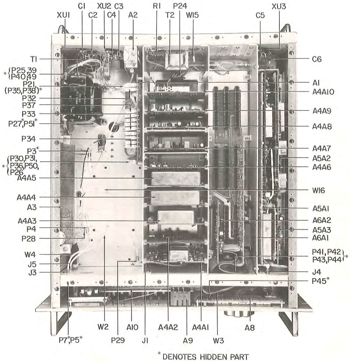
Figure 5-3. WJ-8718 HF Receiver, Top View, Location of Components
