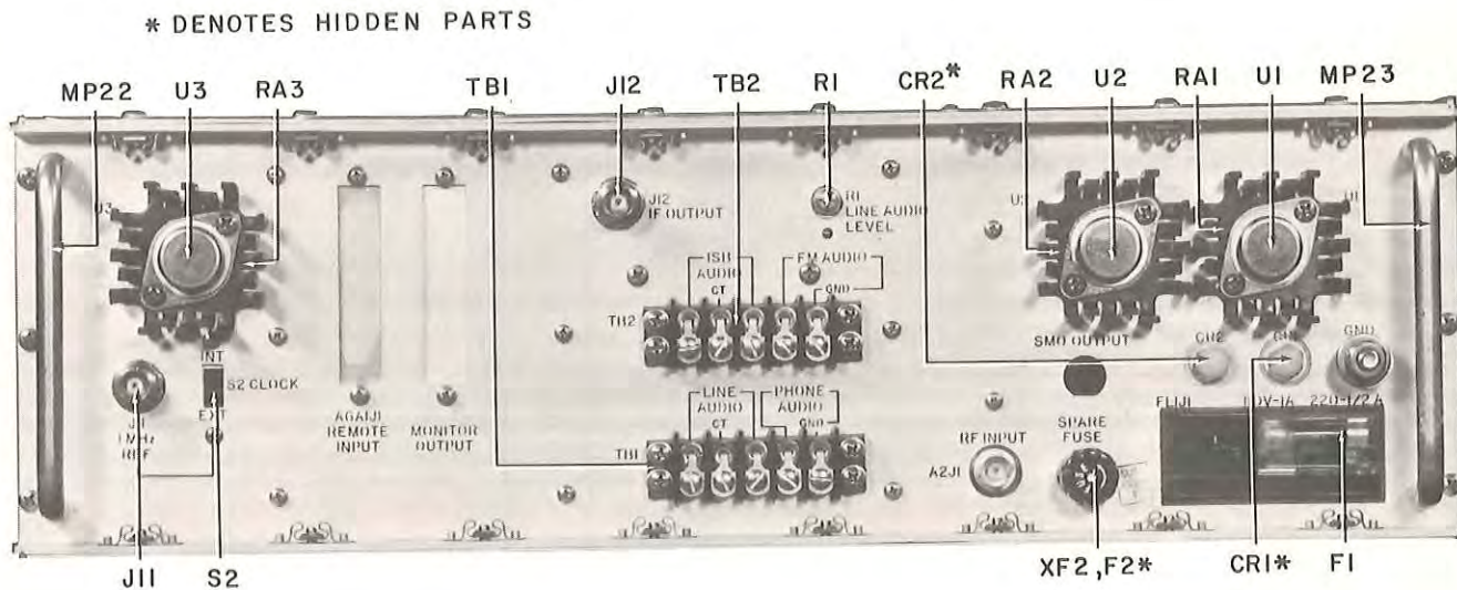
Figure 5-2. WJ-8718 HF Receiver, Rear View, Location of Components
