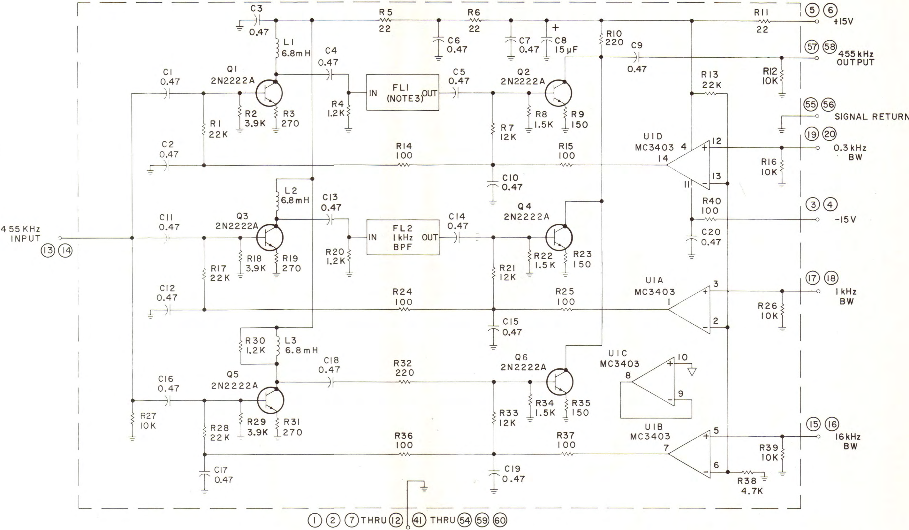
Figure 6-5. Type 791595 455 kHz Filter Switch (A4A3), Schematic Diagram 43561
