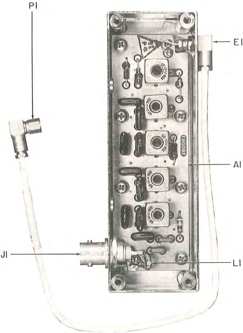
Figure 5-6A. Type 791616 Input Filter (Product Improvement) A2, Location of Components
