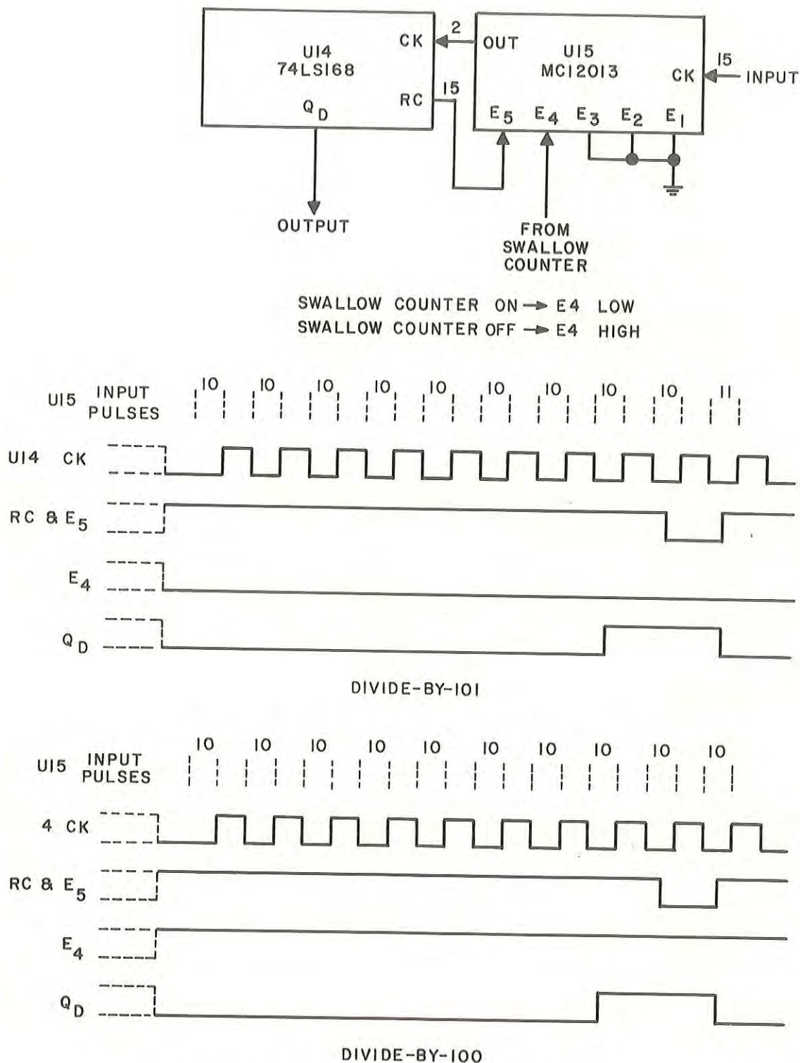
Figure 3-15. 2nd LO Prescaler Timing Diagram
