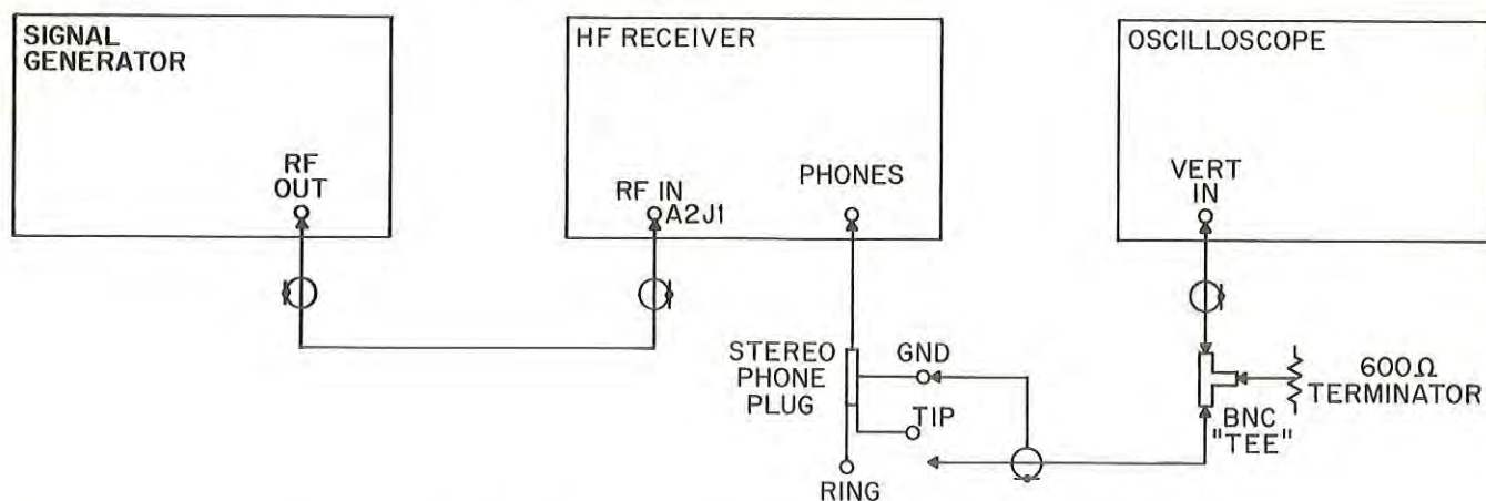
Figure 4-24. ISB Detector/Audio Adjustment, Test Setup
