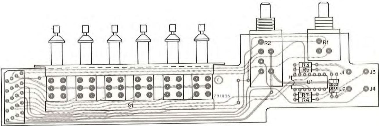
Figure 5-39. Type 791826 Lower Panel Control (A10A2), Location of Components
