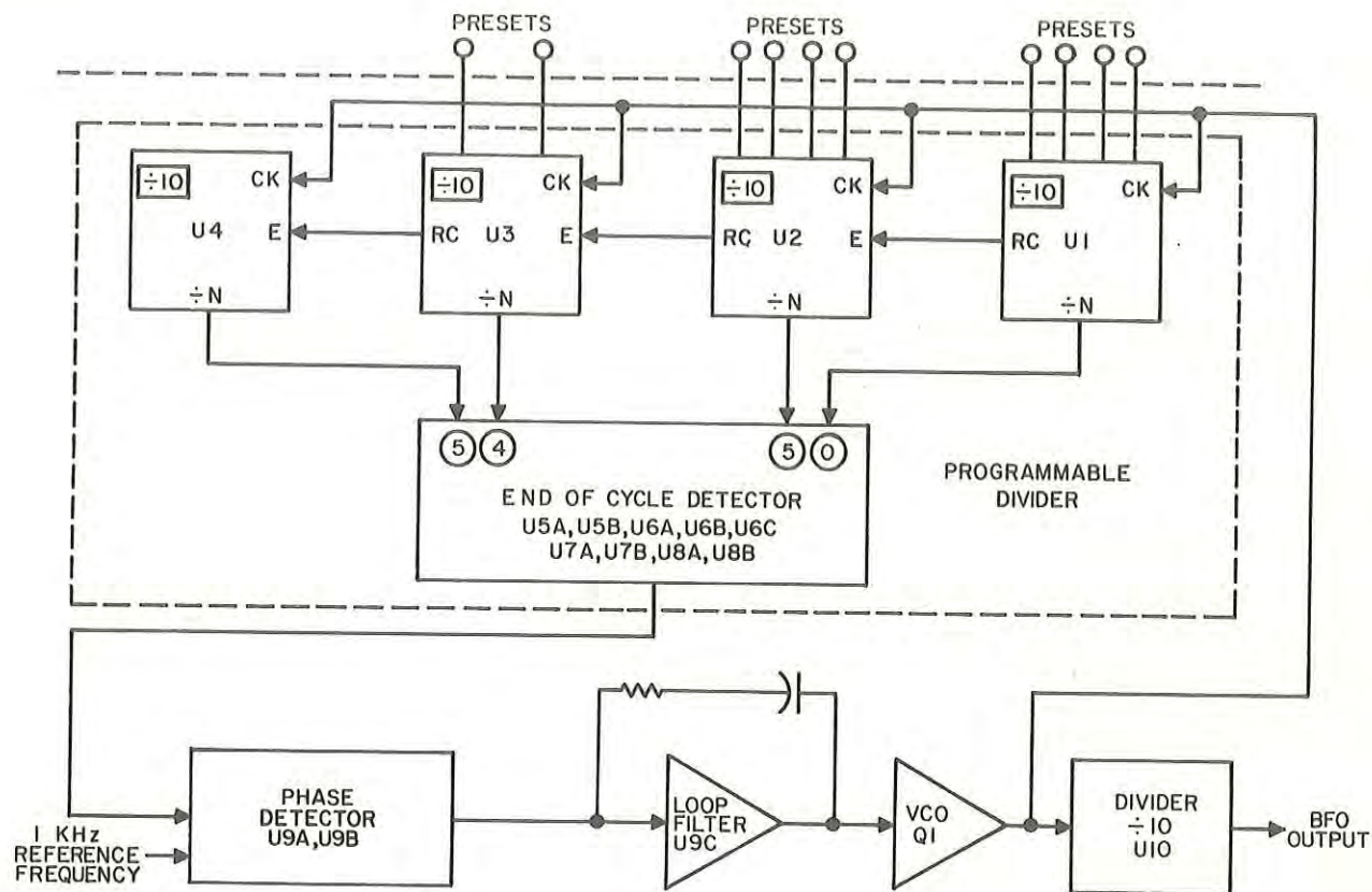
Figure 3-13. BFO Functional Block Diagram
