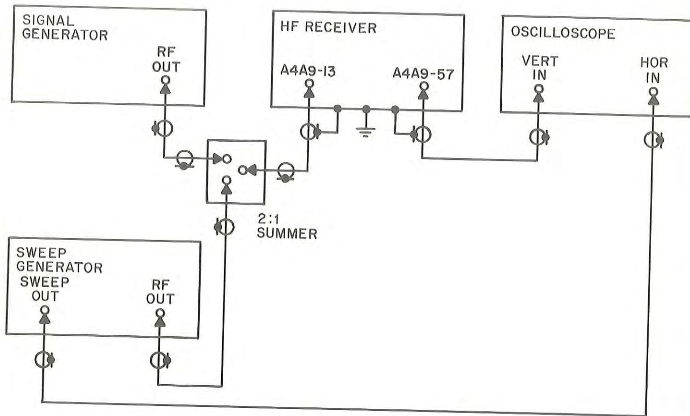
Figure 4-25. FM Discriminator Alignment, Test Setup
