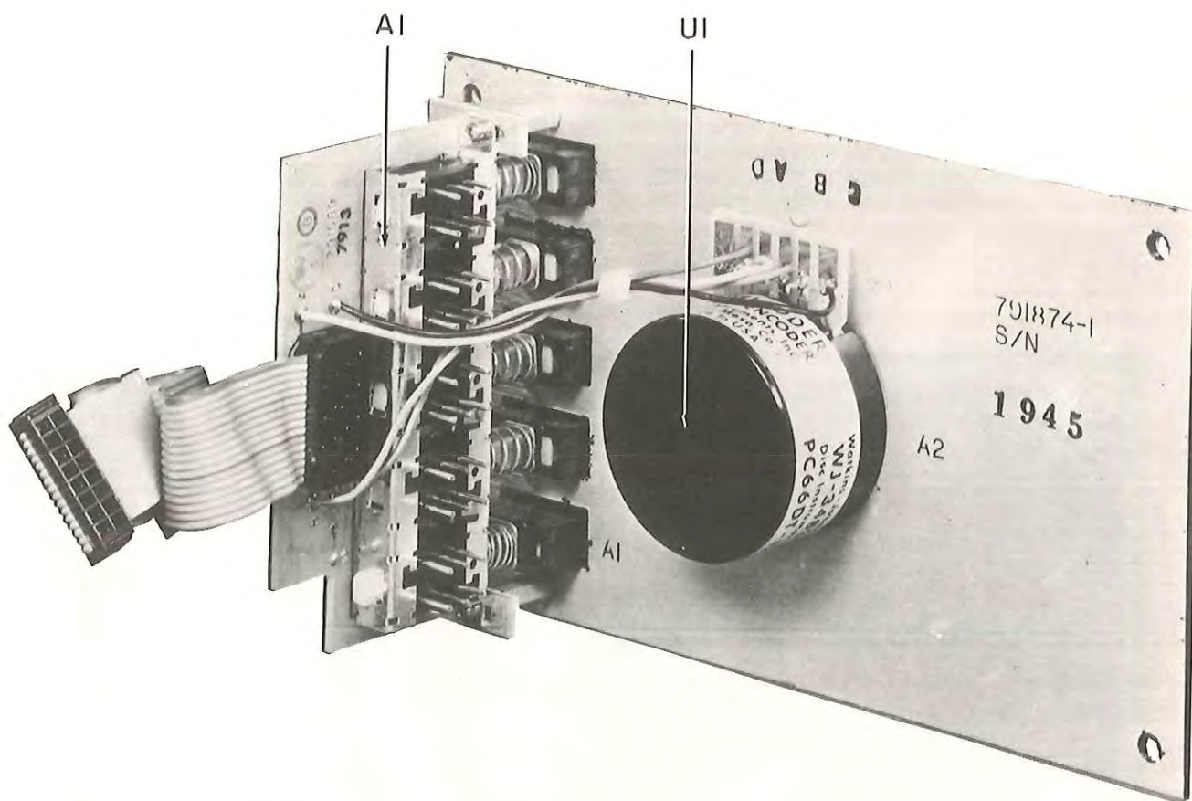
Figure 5-33. Type 791874-1 Manual Tuning Module (A7), Rear View, Location of Components
