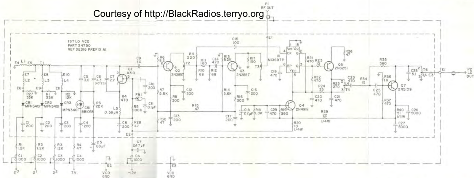
Figure 6-14. Type 791629 Voltage Controlled Oscillator (A5A1A1), Schematic Diagram 51198
