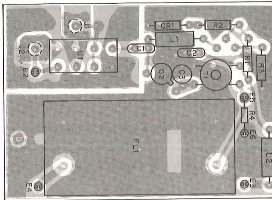
Figure 5-8. Part 34748 1st Mixer, 1st IF (A3A1), Location of Components
