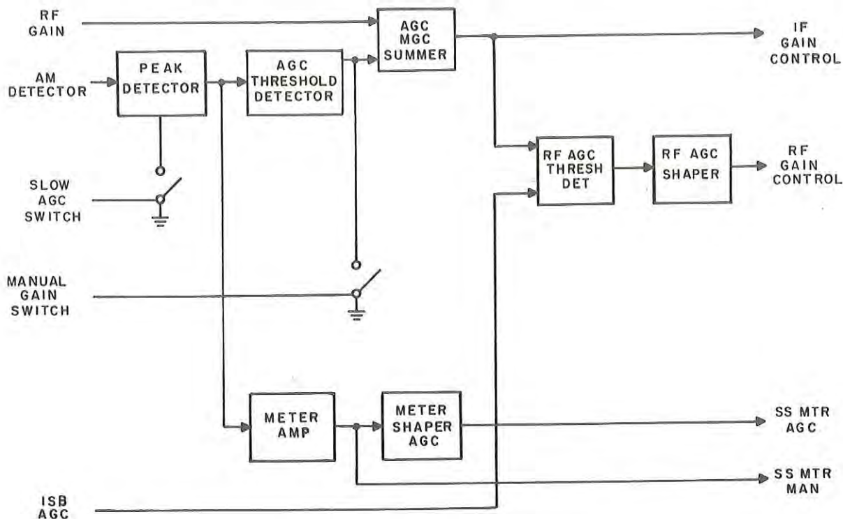
Figure 3-3. Simplified AGC Circuit
