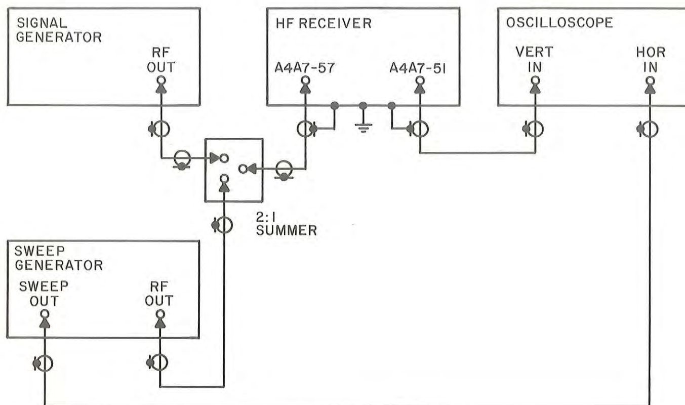
Figure 4-21. 455 kHz Amplifier/AM Detector Response Alignment, Test Setup
