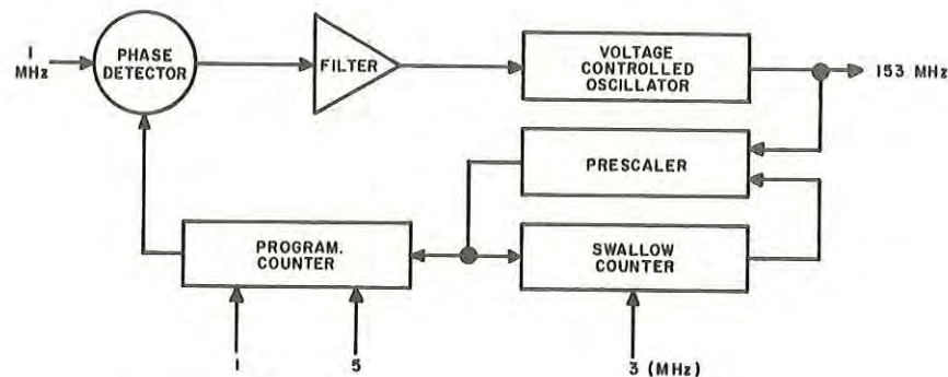
Figure 3-8. Prescaler Dividing Technique
