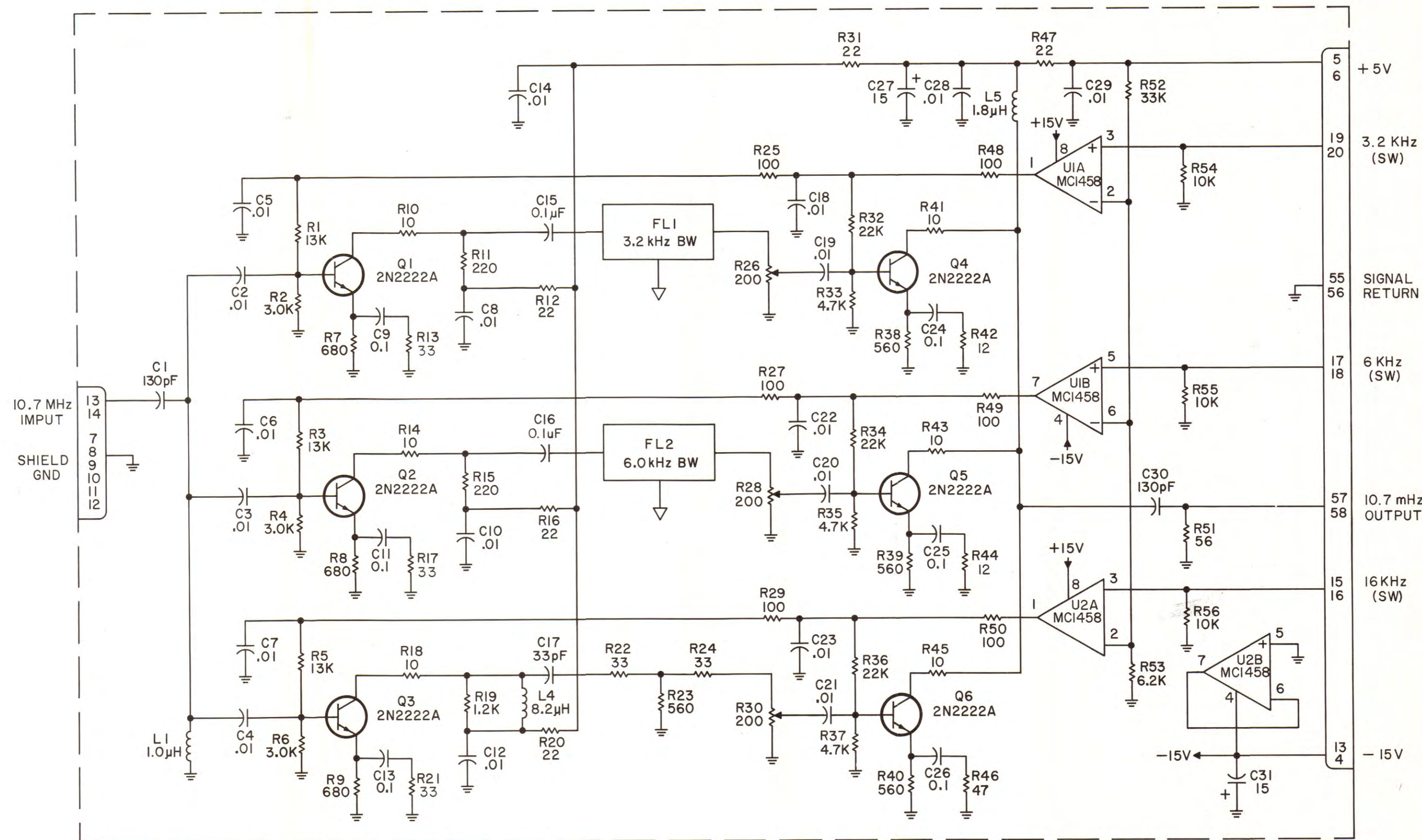
Figure 6-3a. Type 791594 10.7 MHz Filter Switch (A4A1) Schematic Diagram 480103 (Product Improvement)
