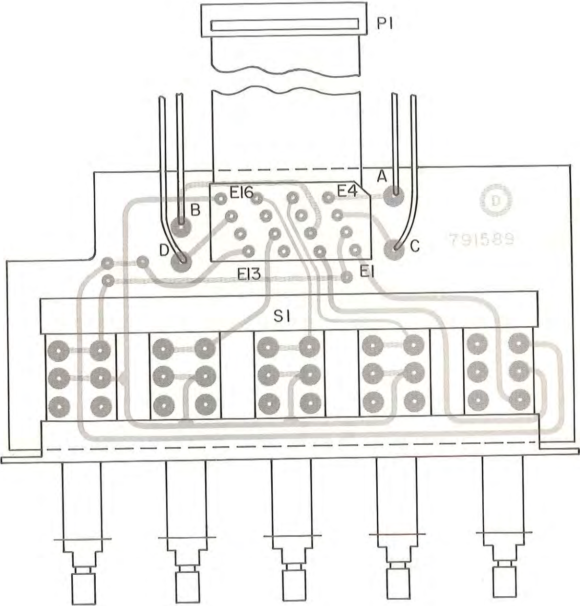
Figure 5-34. Type 791589 Tuning Resolution (A7A1), Location of Components
