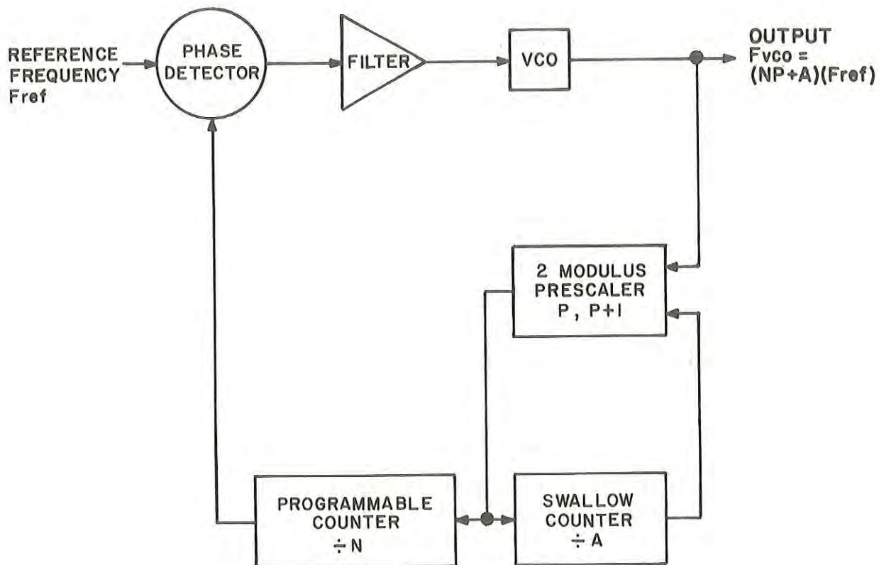
Figure 3-7. Two-Modulus Prescaling in the Phase Lock Loop
