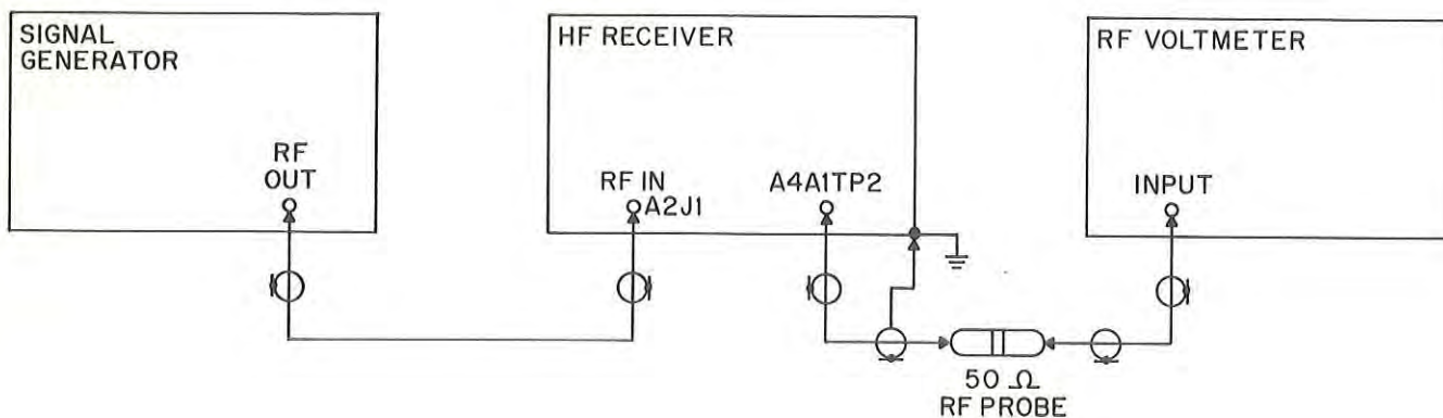
Figure 4-20. 10.7 MHz Filter Switch Adjustment, Test Setup
