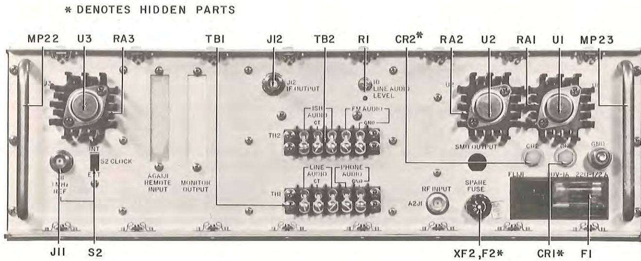
Figure 2-3. WJ-8718 HF Receiver, Rear Panel View
