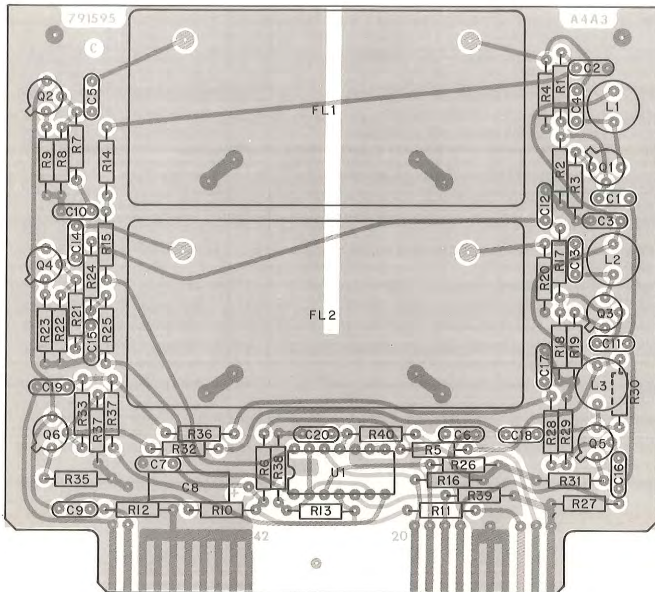
Figure 5-14. Type 791595 455 kHz Filter Switch (A4A3), Location of Components
