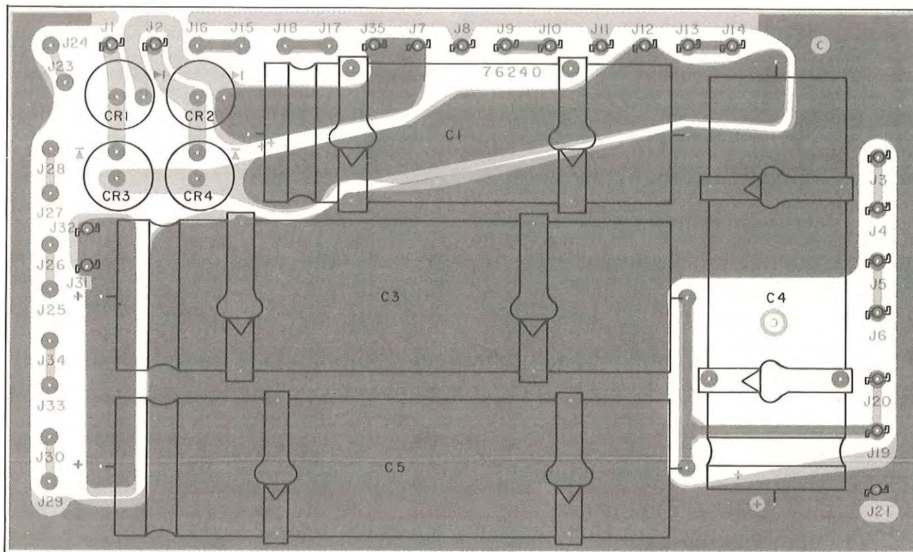
Figure 5-5. Type 76240 Power Distribution (A1), Location of Components
