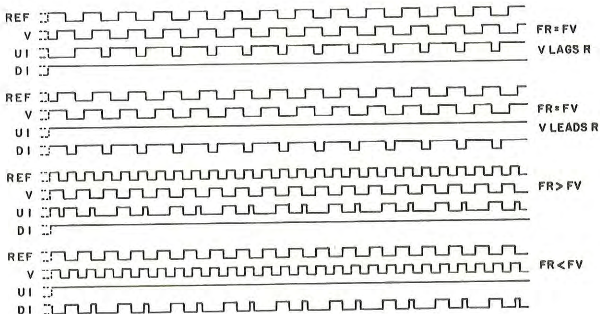
Figure 4-18. Phase Detector Timing Diagram
