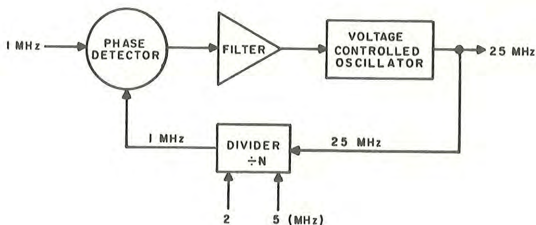
Figure 3-6. Programmable Phase Lock Loop
