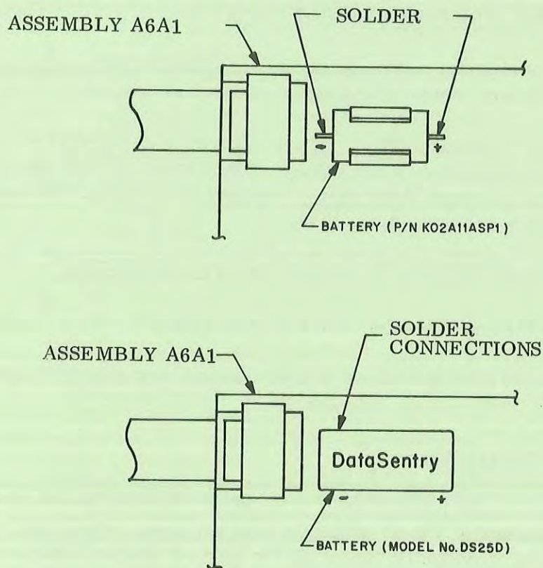
Figure 1. BATTERY A6A1BT1 INSTALLATION
