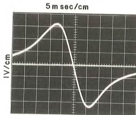
Figure 4-26. FM Discriminator Alignment, Typical Response
