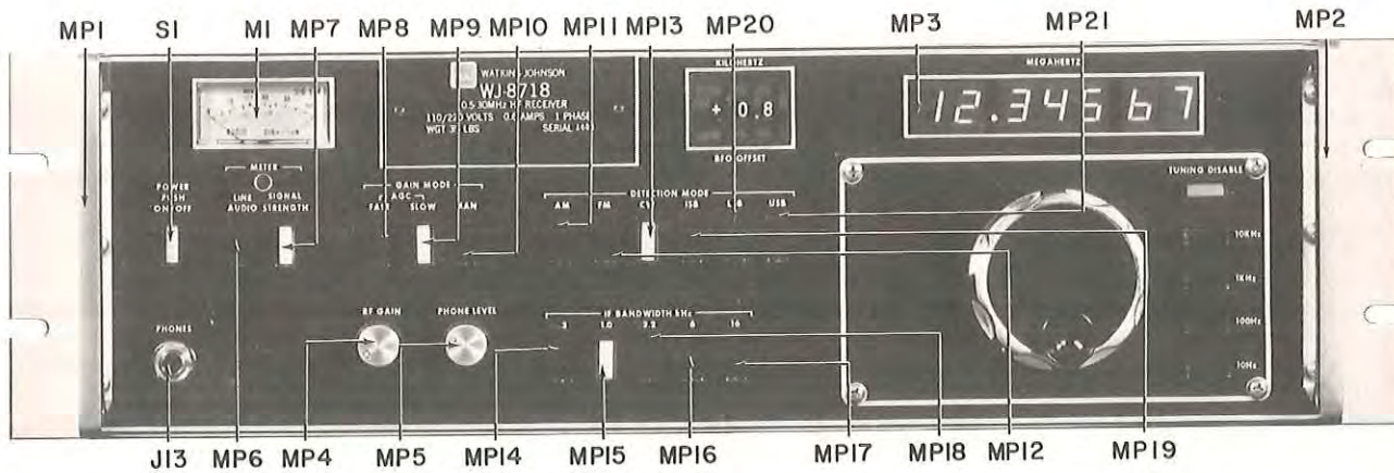
Figure 5-1. WJ-8718 HF Receiver, Front Panel, Location of Components
